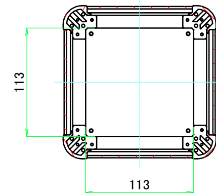
C-C (1:4)
